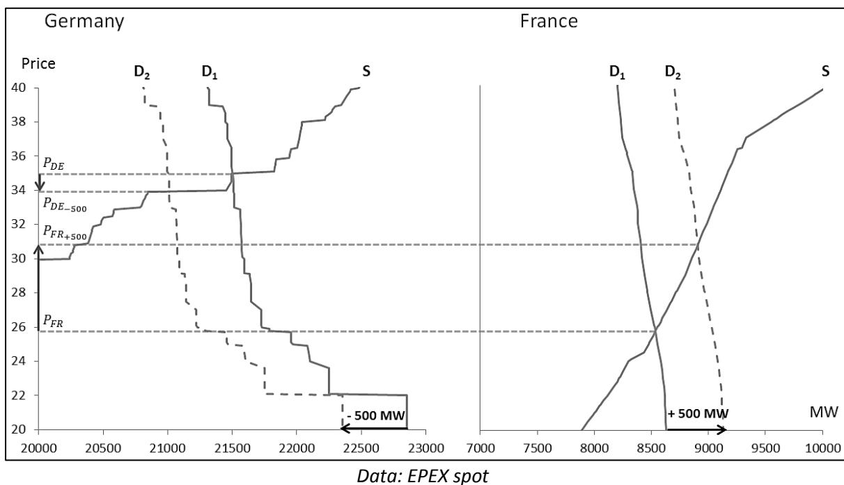
Figure 2: Market resilience for a 500MW demand variation in France and Germany on the 05/05/2013 at 10pm.
