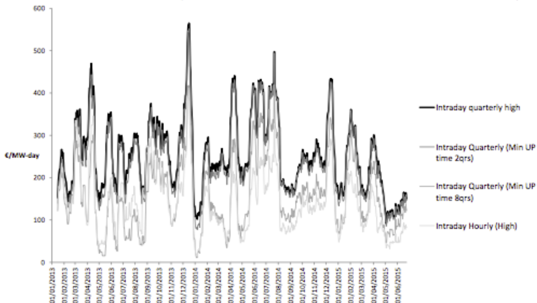
Figure 6: IDM quarterly theoretical net revenues for a 1MW CCGT under different minimum up-time durations (source: own calculations based on EPEX SPOT, ICE).
