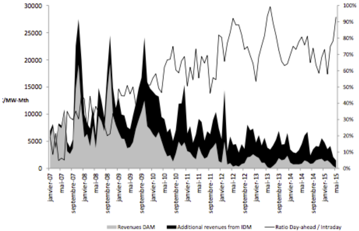
Figure 4: DAM/IDM theoretical net revenues for a 1MW perfect CCGT
