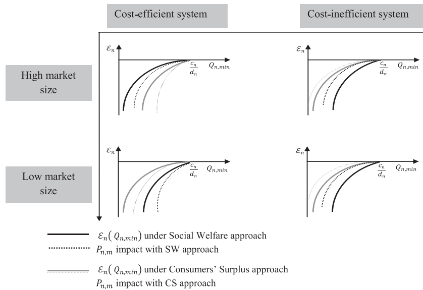
Fig. 5. Elasticity of demand and optimal consumption reduction.
