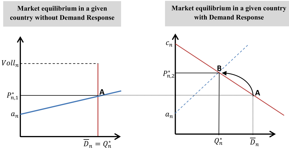
Fig. 1. Impact of a DR program on market equilibrium.
