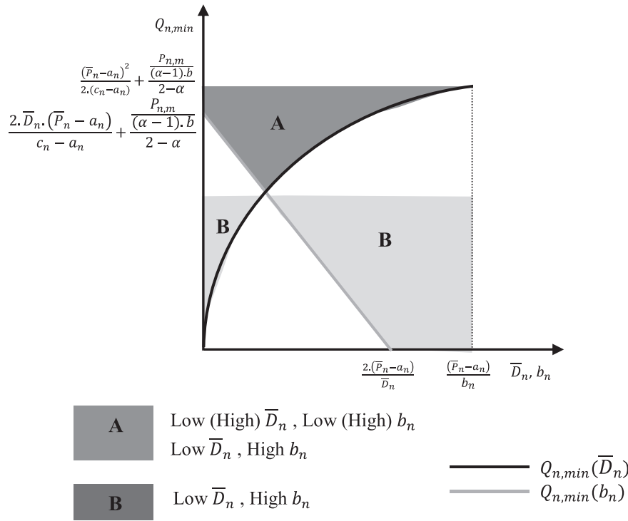
Fig. 2. Optimal regions of DR for efficient country.
