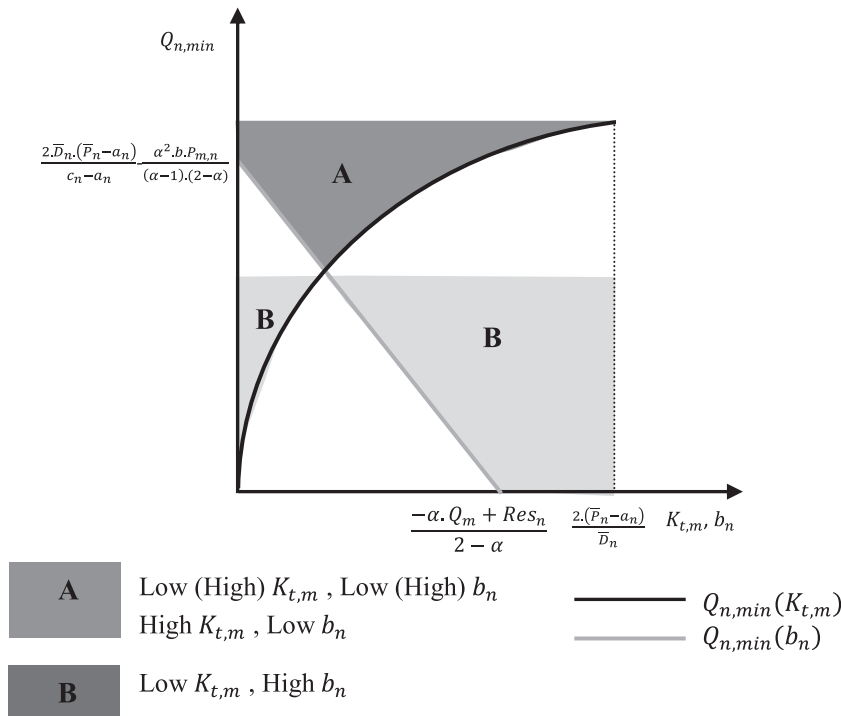
Fig. 3. Optimal regions of DR for inefficient country.
