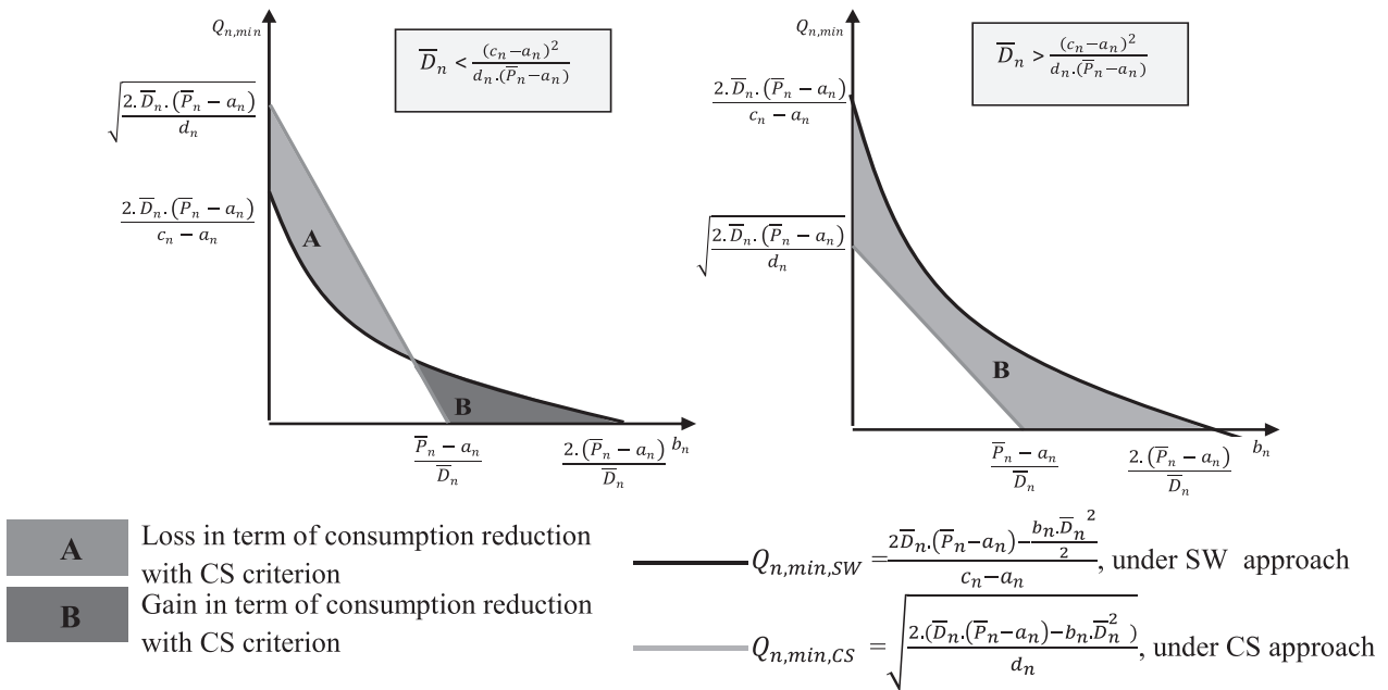
Fig. 4. Maximal consumption reduction under consumers' surplus criterion and social welfare criterion.
